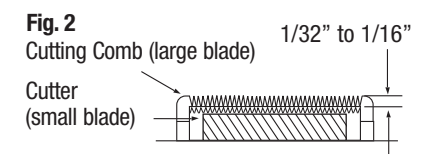
Fig. 2 Cutting Comb (large blade) 1/32" to 1/16" Cutter (small blade)
